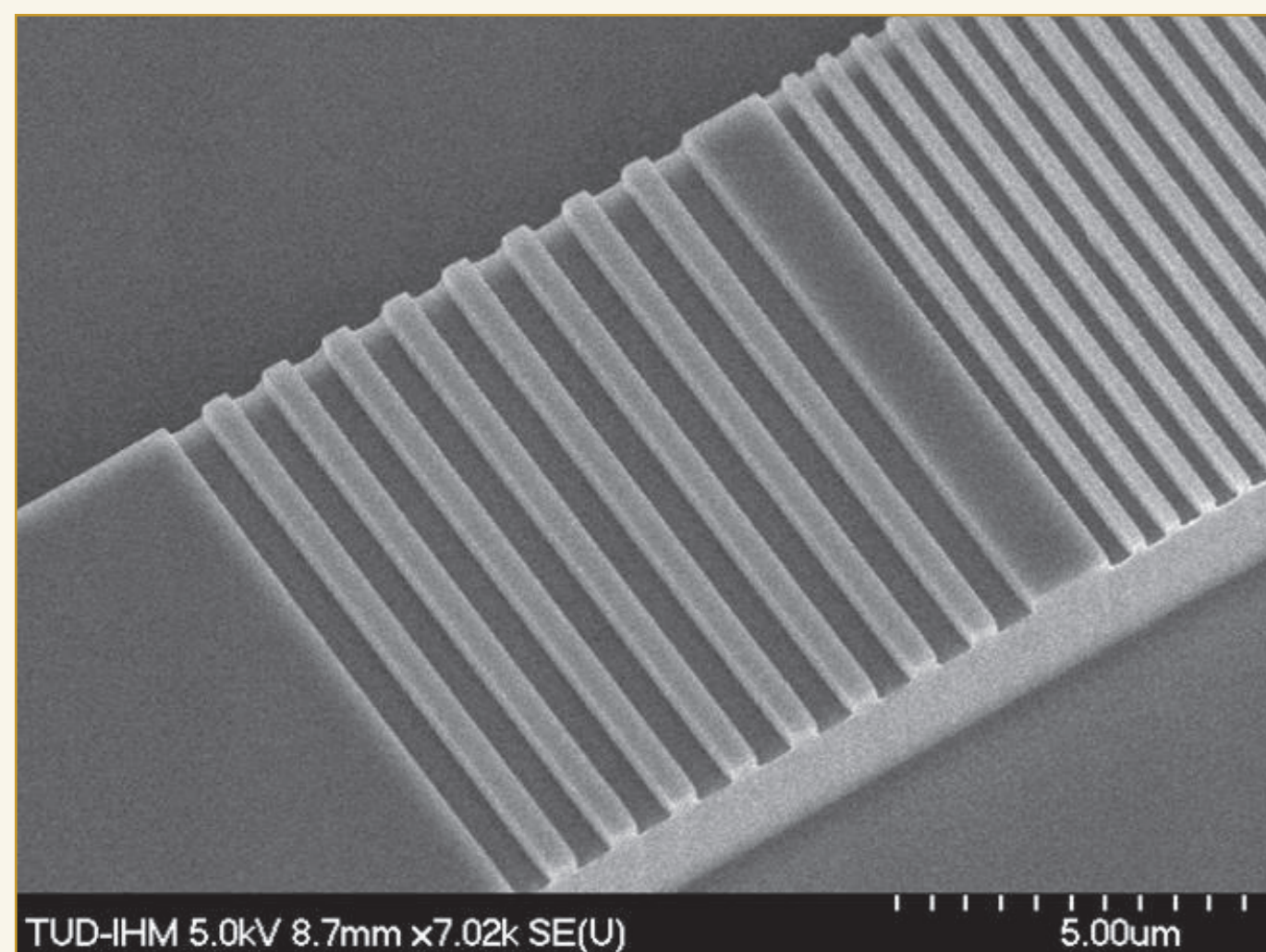
Patterned OrmoCore waveguide, fabricated via UV imprint (Courtesy of TU Dresden, Germany)
