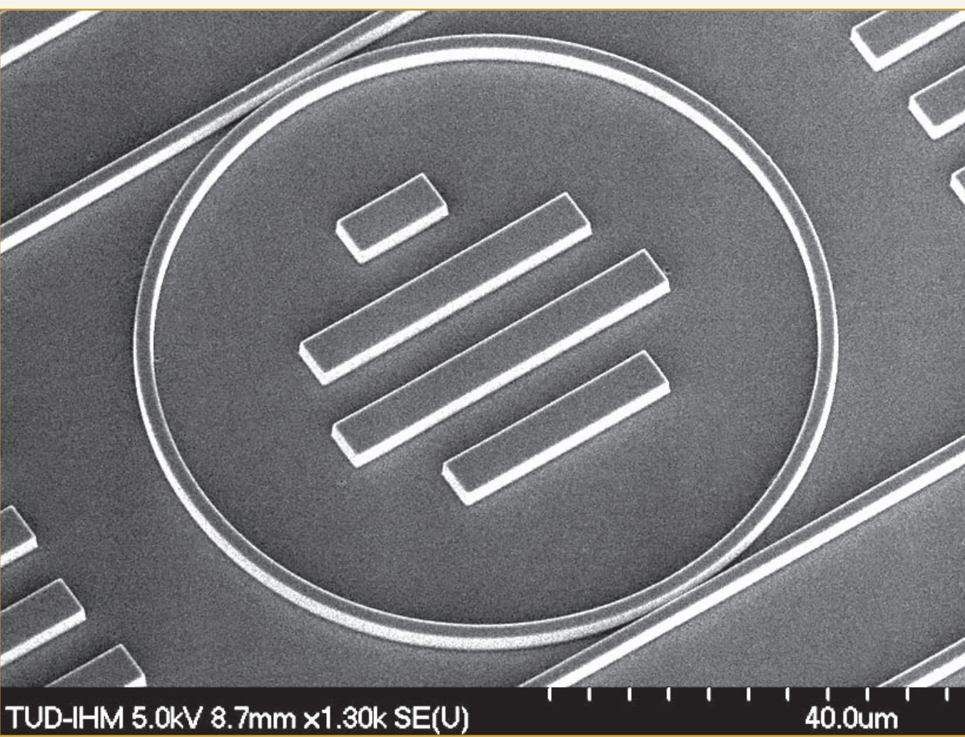
Replicated OrmoCore microring resonator (courtesy of TU Dresden, Germany)
