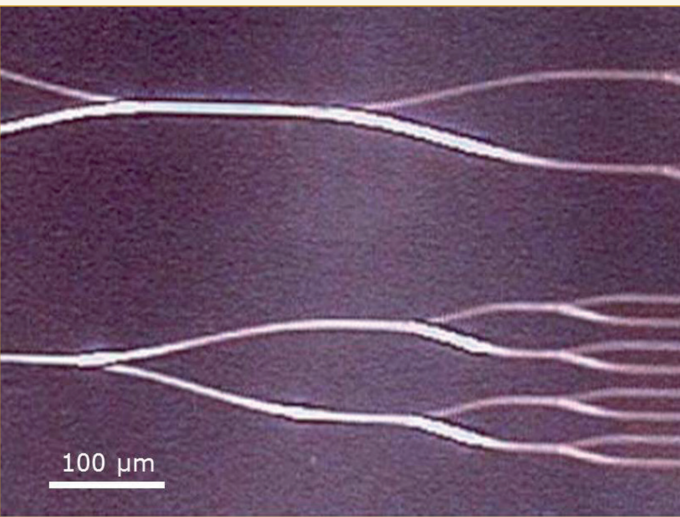
OrmoClad/OrmoCore with 8 μm waveguide coupling structure on lower cladding
