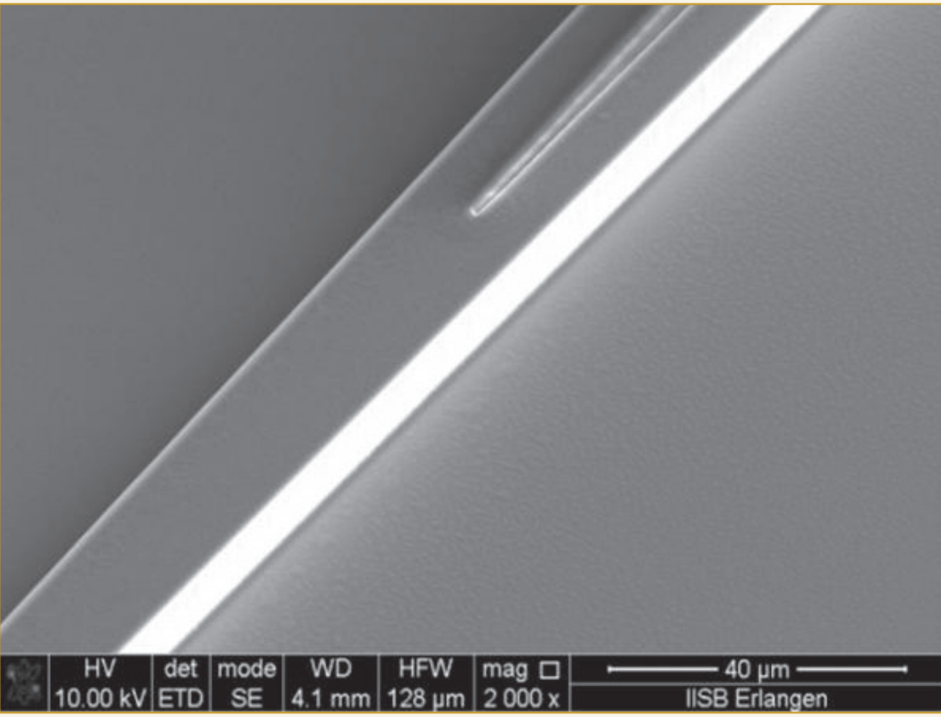
OrmoCore Y-coupler element, fabricated via UV imprint (Courtesy of FhG IISB, Germany)
