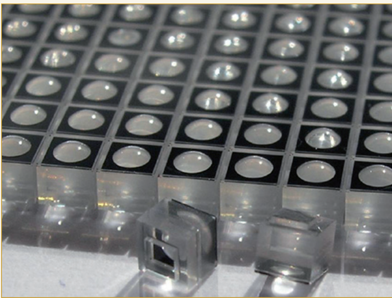
Mass-manufactured OrmoComp® micro lenses (1.3 mm diameter, 250 µm height) on glass (courtesy of FhG IOF, Germany)
